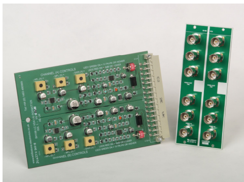
BH193/196 (left) and integrated in a BH220 (above)
